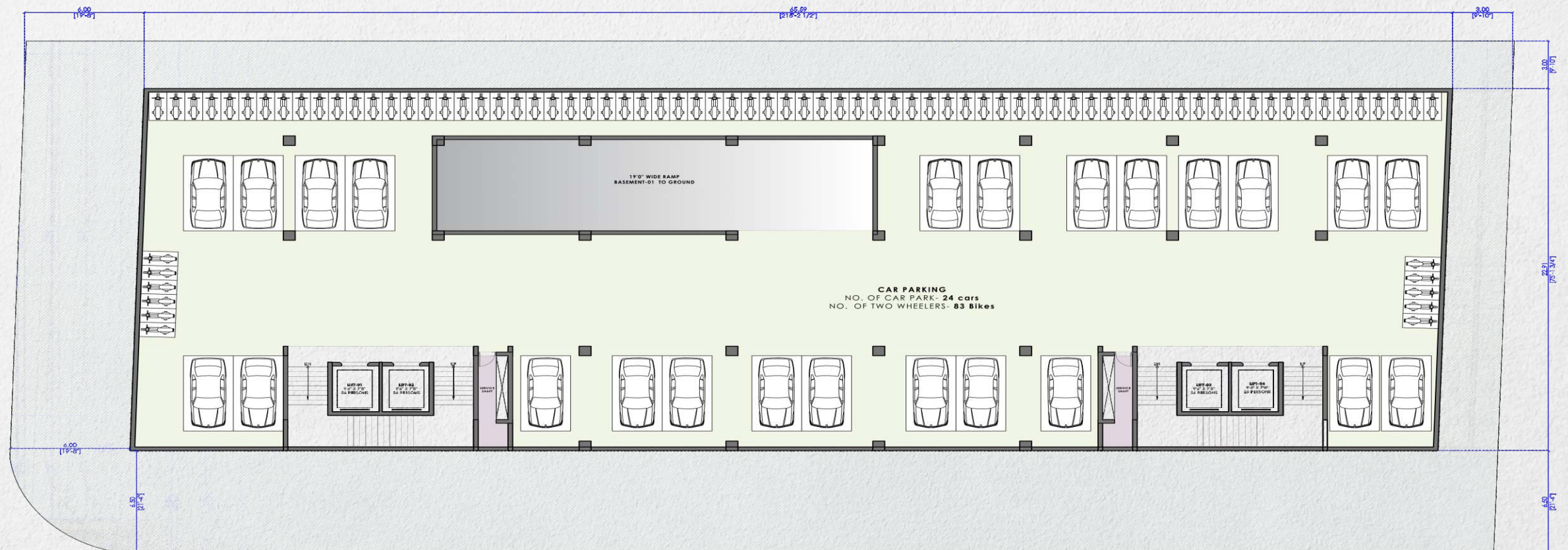
BASEMENT FLOOR PLAN CONSTRUCTION AREA 1470.12 SQ.MT ( 15824.37 SQ.FT. )
